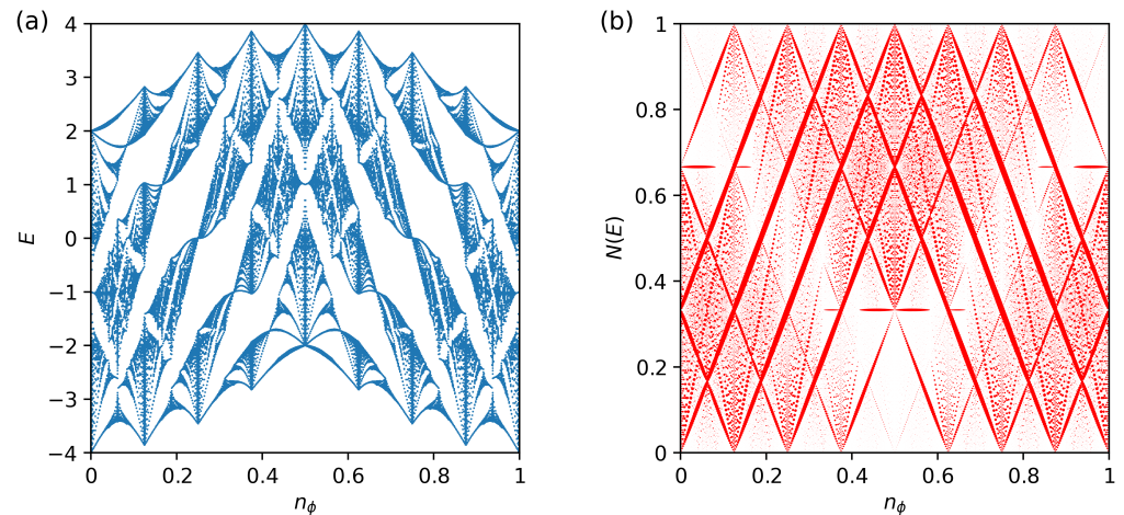
Figure 4: Kagome Lattice (a) Hofstadter butterfly and (b) Wannier diagram for the Hofstadter model defined with nearest-neighbor hoppings on the kagome lattice. (Jing-Min, 2009)
