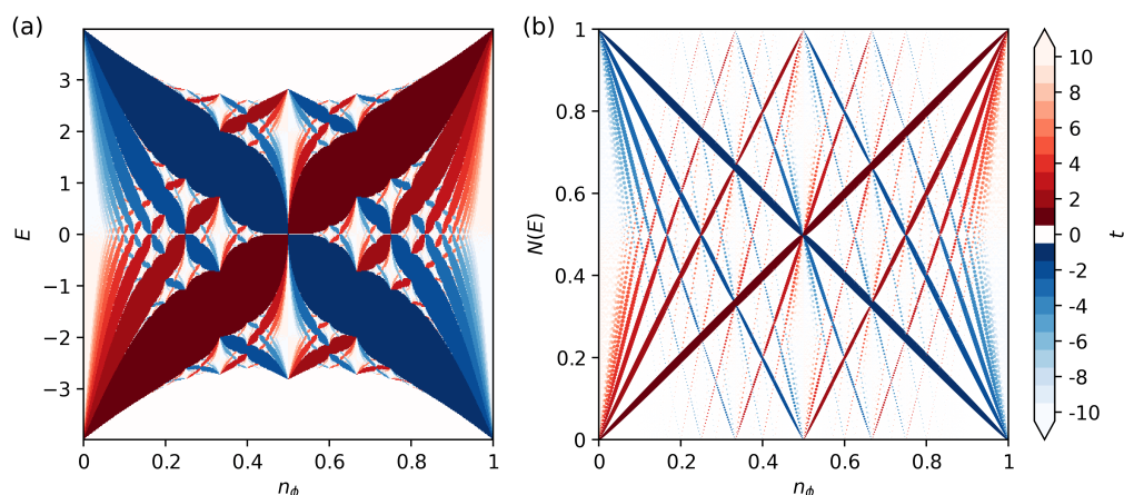
Figure 1: Square Lattice (a) Hofstadter butterfly and (b) Wannier diagram for the Hofstadter model defined with nearest-neighbor hoppings on the square lattice. (a) The energy E , and (b) the integrated density of states below the gap N(E) , are plotted as a function of flux density n_\phi = BA_{\min}/\phi_0 = p/499 , where B is the perpendicular field strength, A_{\min} is the area of a minimal hopping plaquette, \phi_0 is the flux quantum, and p is an integer. The r -th gap is colored with respect to t = \sum_{i=0}^r C_i , where C_i is the Chern number of band i . The size of the points in the Wannier diagram is proportional to the size of the gaps. (Colandrea et al., 2022)
