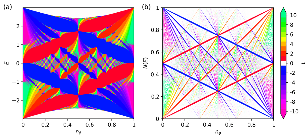
Figure 3: Honeycomb Lattice (a) Hofstadter butterfly and (b) Wannier diagram for the Hofstadter model defined with nearest-neighbor hoppings on the honeycomb lattice. (Agazzi et al., 2014)
