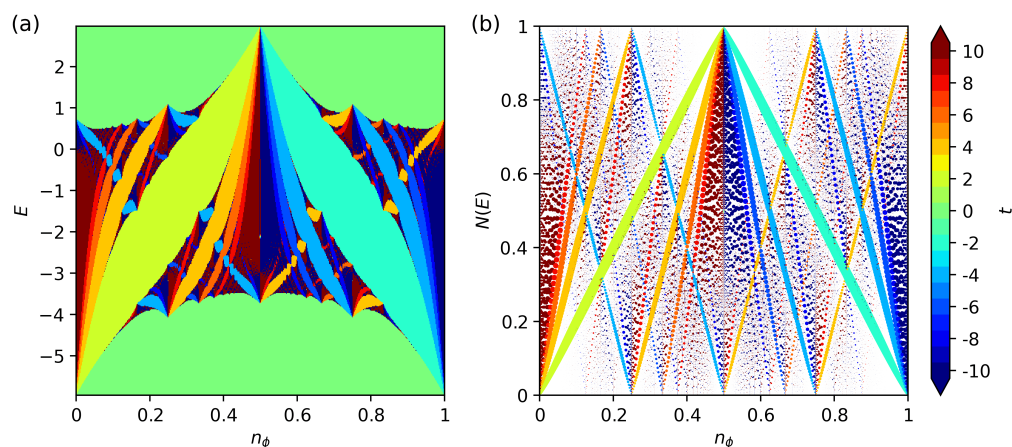
Figure 2: Triangular Lattice (a) Hofstadter butterfly and (b) Wannier diagram for the Hofstadter model defined with nearest-neighbor hoppings on the triangular lattice. (Avron et al., 2014)
