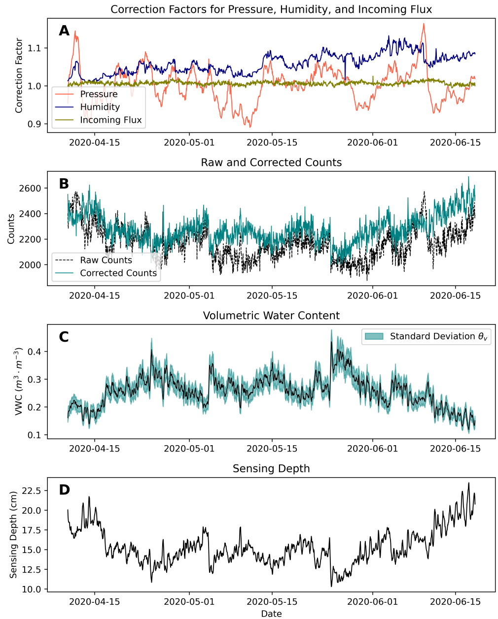
Figure 3: Outputs of a stationary device in each of the steps of the workflow, A) Impact of each factor in the correction process. B) Difference between raw and corrected counts. C) Resulting volumetric water content time series with the propagated neutron count uncertainty. D) Depth that accounts for the 86% of the observed counts.
