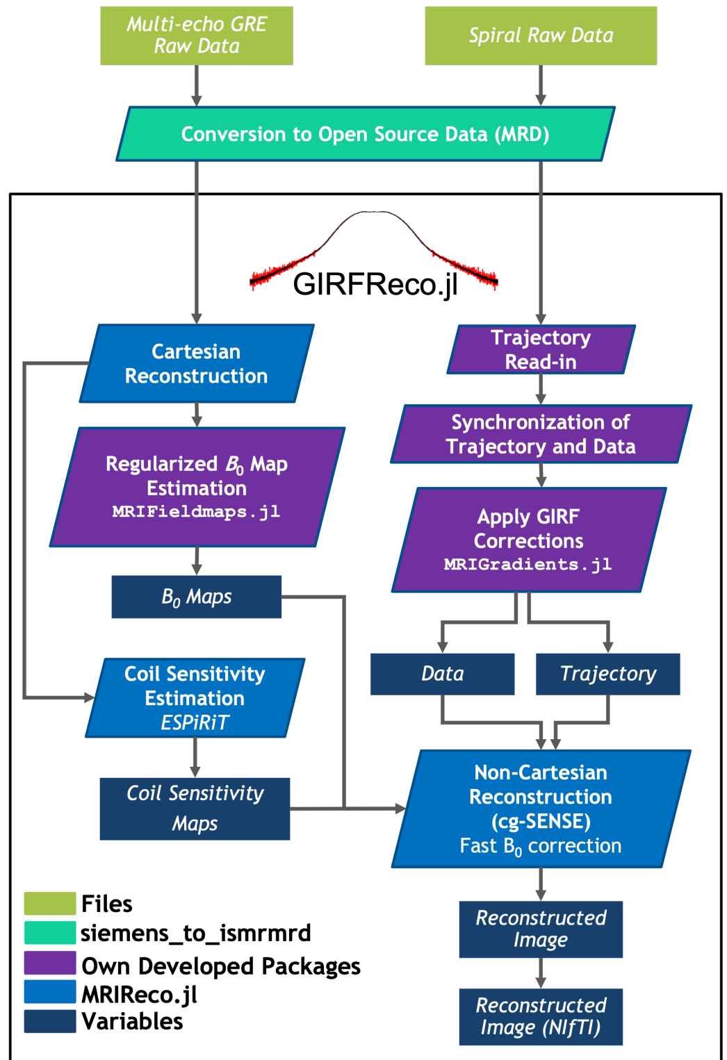
Figure 1. Overview of the GIRFReco.jl signal processing and reconstruction pipeline. Depicted is the workflow from raw acquired k -space data to the final reconstructed images with the respective tasks (parallelogram), in/output data (rectangles) and the location of the processing components within different packages (colours).
