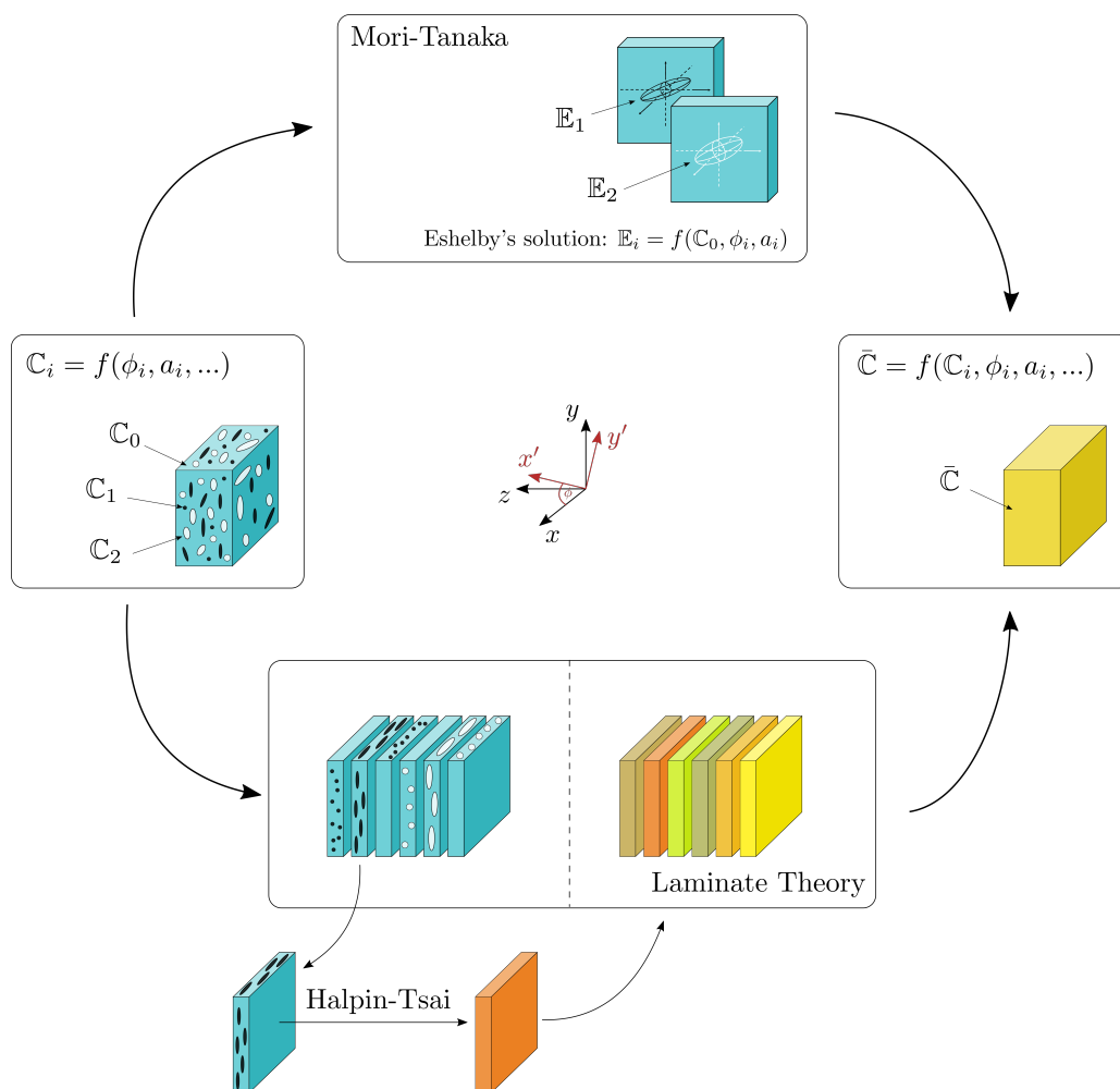
Figure 2: Schematic of implemented homogenization methods, where C_i is the stiffness tensor of component i , \bar{C} is the effective stiffness tensor, \phi_i is the orientation angle of fiber i and a_i its aspect ratio. Illustration in reference to Fu & Lauke (1998b).
