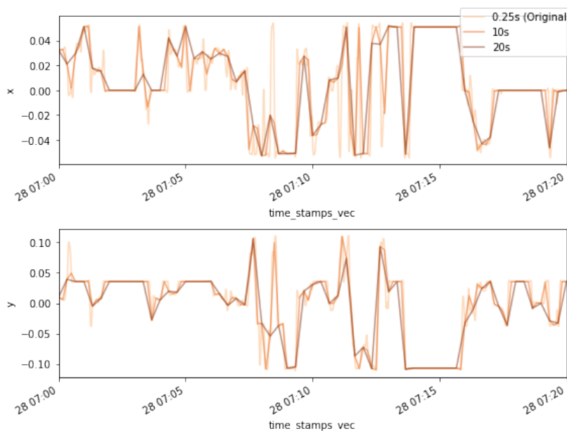
Figure 4: Resampling trajectories by different time scales is performed with resample_time .
