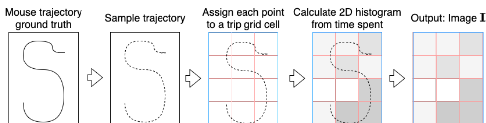
Figure 2: Trip grid image generation from mouse trajectory.
