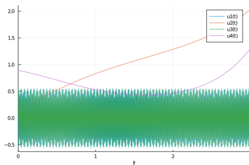
Figure 1: Hénon-Heiles solution.
